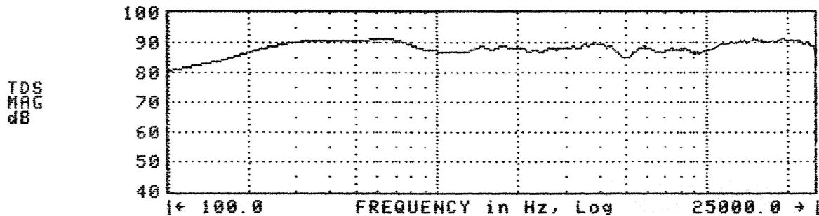
Frequency Magnitude Response @ 2.83V//1Meter
