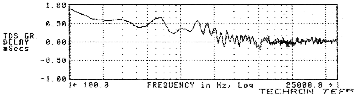
Group Delay Response @ 1Meter
